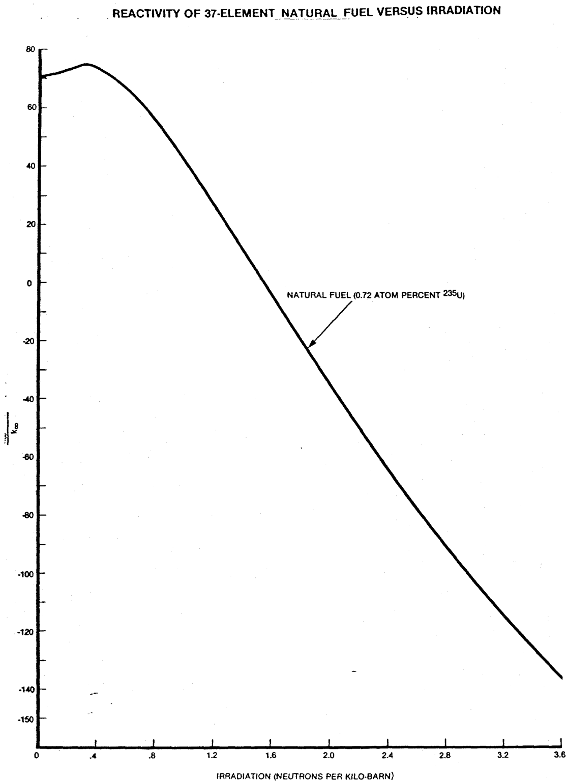
Figure 5.2 Infinite-Lattice Multiplication Constant for Standard CANDU-6 Lattice Fuelled with Natural Uranium
